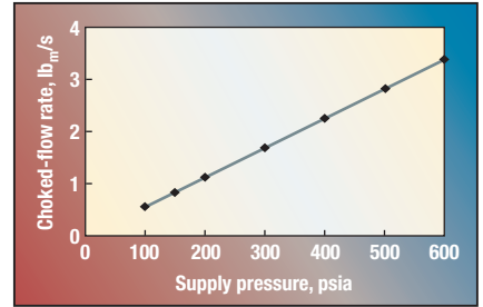
FIGURE 4. Increasing the supply pressure raises the choked flowrate (shown here for an adiabatic flow of steam)
